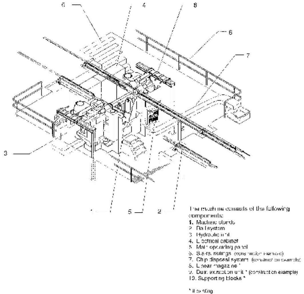
Fig. 20.1.5.1: 3D-view of the Hegenscheidt U2000 underfloor wheel lathe.
