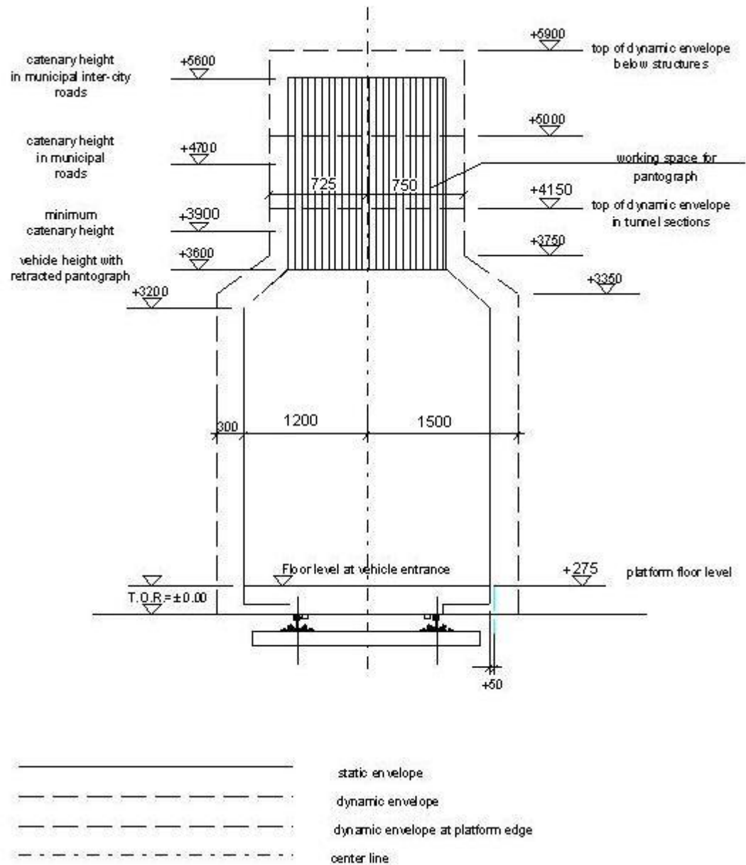
Fig. 20.3.1: Static and dynamic vehicle envelope
