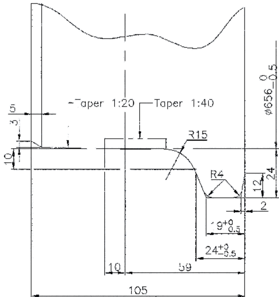
Fig. 20.1.6.1: Current wheel profile
