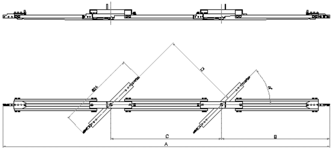
Fig. 20.2.8.2: Elektroline Series 265-XXX. Electrical discontinuity for tram
