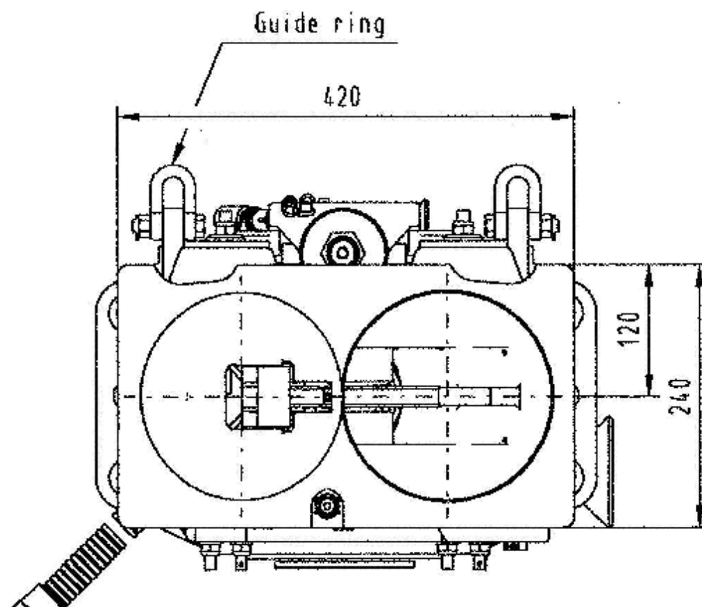
Fig. 20.1.8.1: Side and front views of the automatic coupler for the existing vehicles (371 Dellner)
