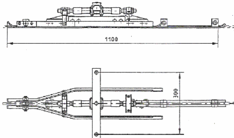
Fig. 20.2.6.1: Section insulator for the lines
