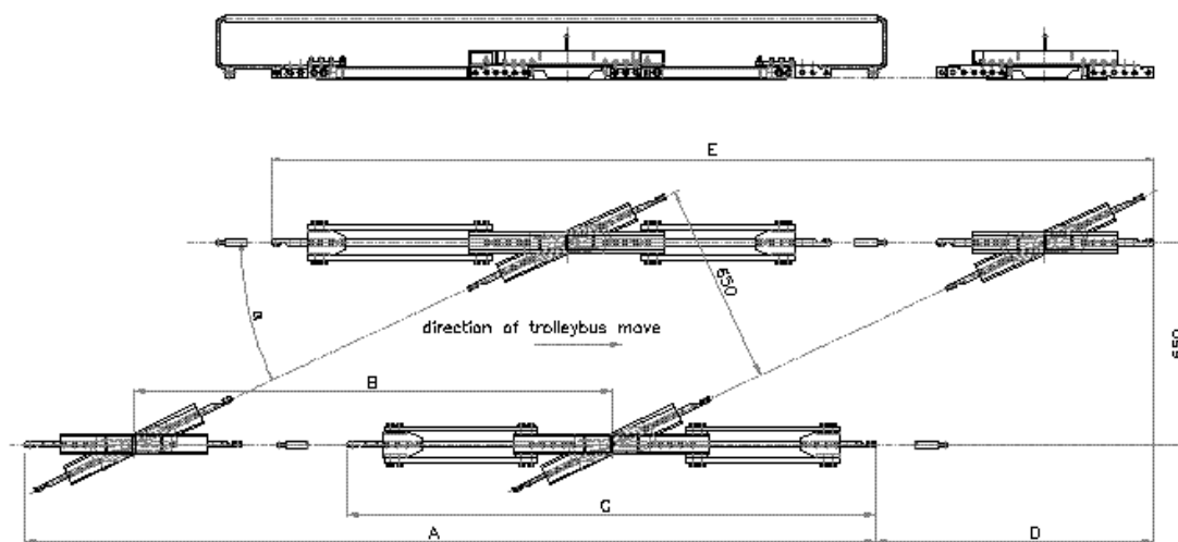
Fig. 20.2.8.1: Elektroline Series 262-XXX. Electrical continuity for tram
